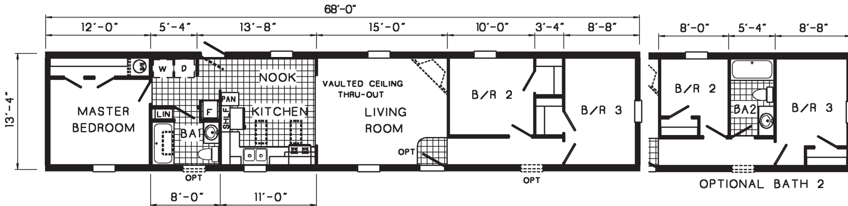
4A109-A 1468 APPROX. 907 SQ. FT.
